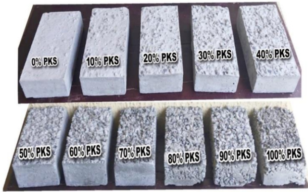
Figure 1: Eleven (11) samples of concrete interlocks with varying percentage ratios of PKS
