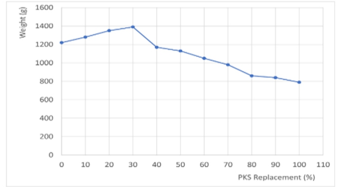
Figure 2: Weight of concrete interlocks versus varying ratios of PKS with GNC
